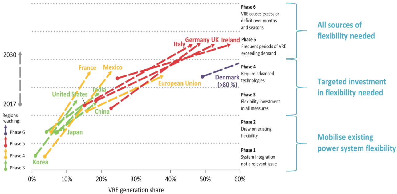
Phases of integration with variable renewables share, 2030
