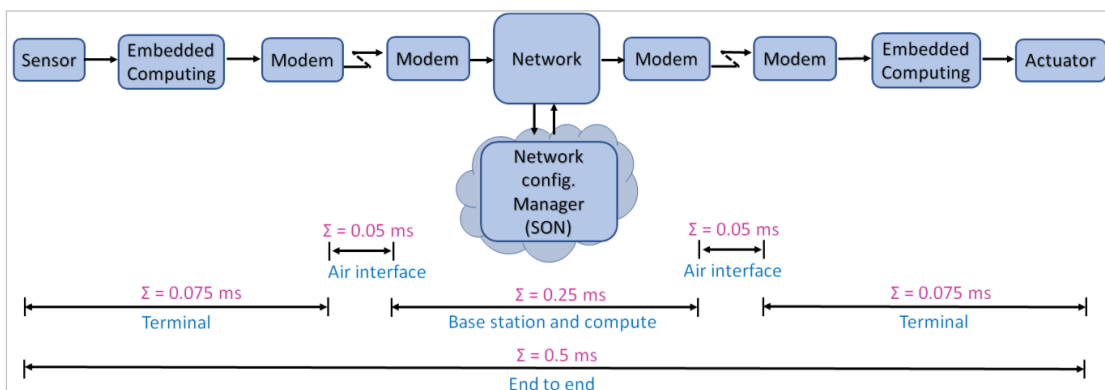
Figure 2-26: Tactile Internet latency requirement
