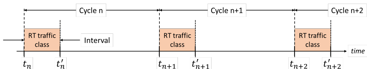
Figure 2-23: Example for time-aware scheduling with absolute time bounds
