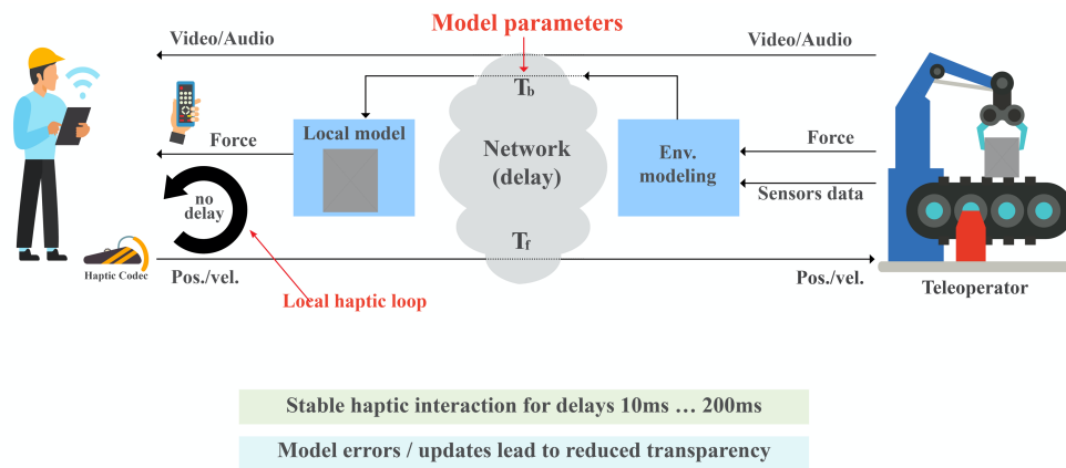
Figure 3-1 Tactile IoT model (Source: adapted from Prof Ekehard Steinbach, TU Munich)
