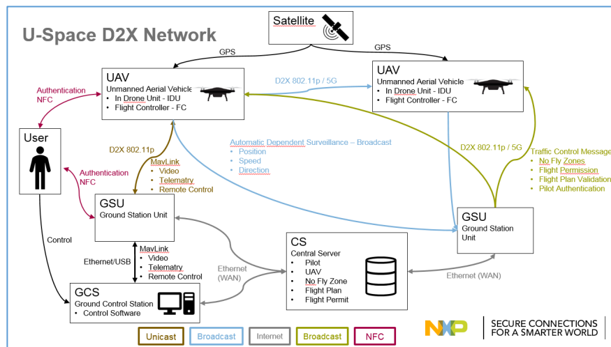
Figure 2-14: UAS operation in U-Space - High level illustration
