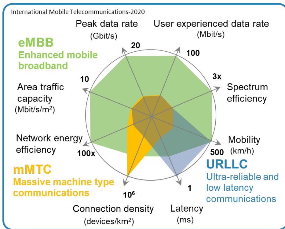
Figure 3-5: 5G technologies heterogeneous requirements
