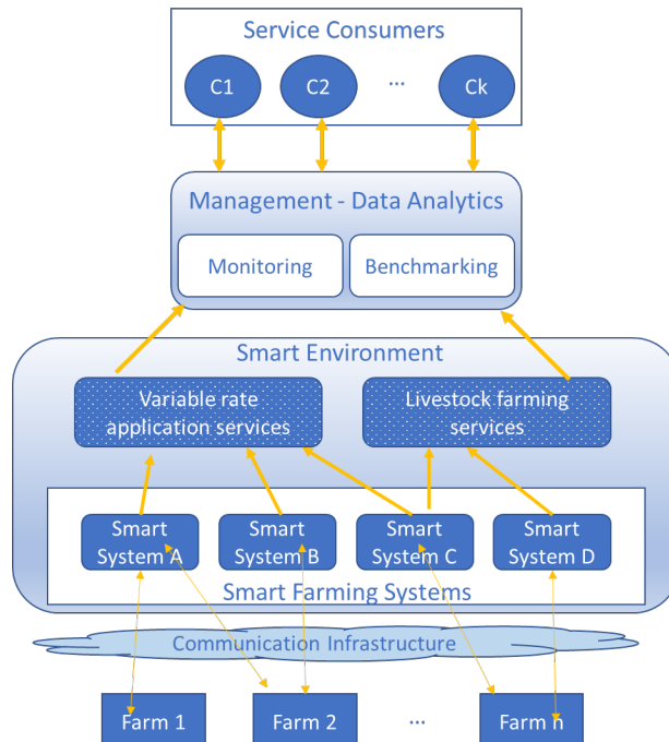
Figure 2-20: Example of a System-of-systems to an IoT based a data-centric livestock farm management
