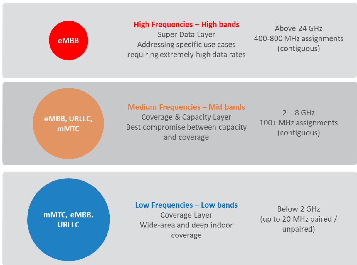
Figure 3-6: Three ranges of the frequency spectrum for 5G technologies
