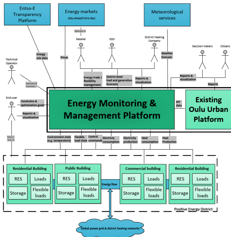
Figure 2-16: Energy monitoring and data flow of the Making-City project for automation and home display – Case of Oulu city. [45] D2.20 – Services and Modules for Oulu ICT Platform.
