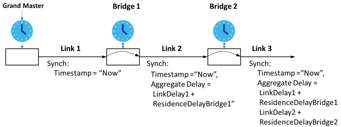
Figure 2-22: IEEE 802.1AS clock synchronization
