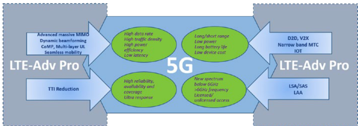
Figure 2-21: LTE-Advanced Pro features and 5G requirements [9]
